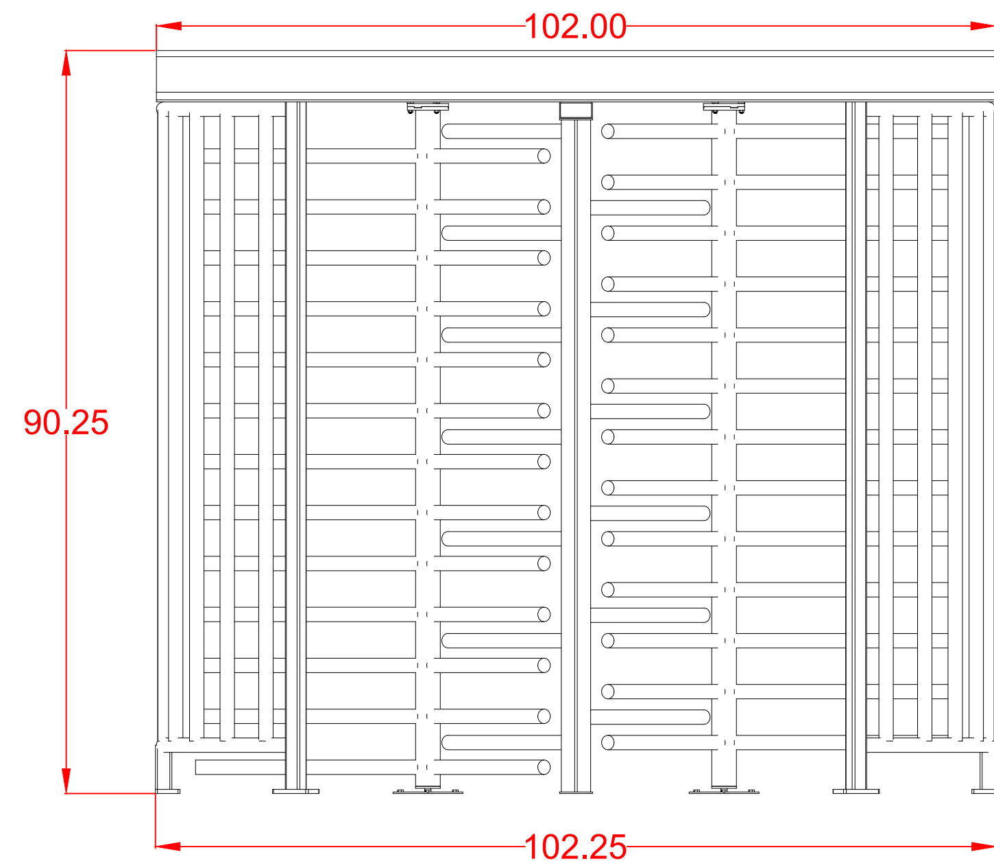
TOP VIEW
