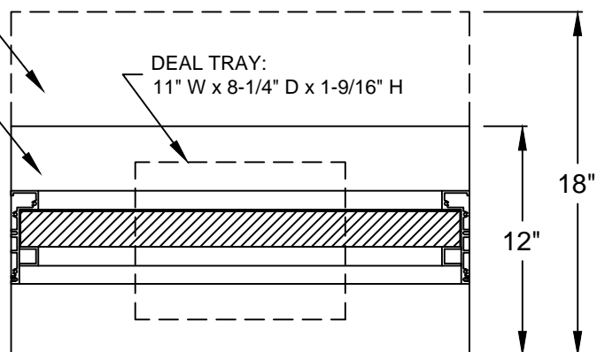
HORIZONTAL SECTION
