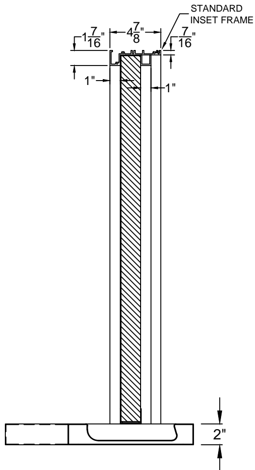
VERTICAL SECTION
